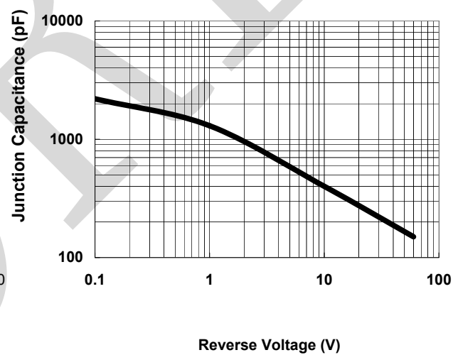
Typical Junction Capacitance Per Diode
