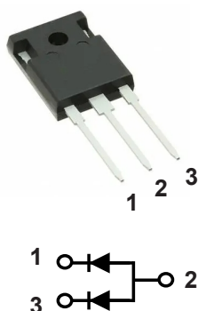
TO-247 MUR6040PTR
